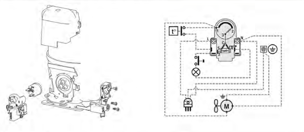
SM01 - EMT/NE SERIES RSCR PTC European Version
