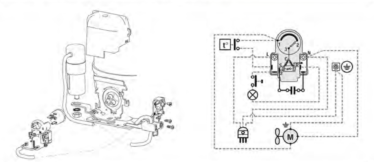
SM02 - EMT/NE SERIES RSCR TSD European Version
