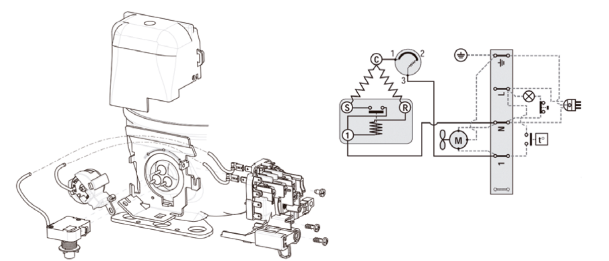
SM04 - EMT/NE SERIES CSIR American Version
