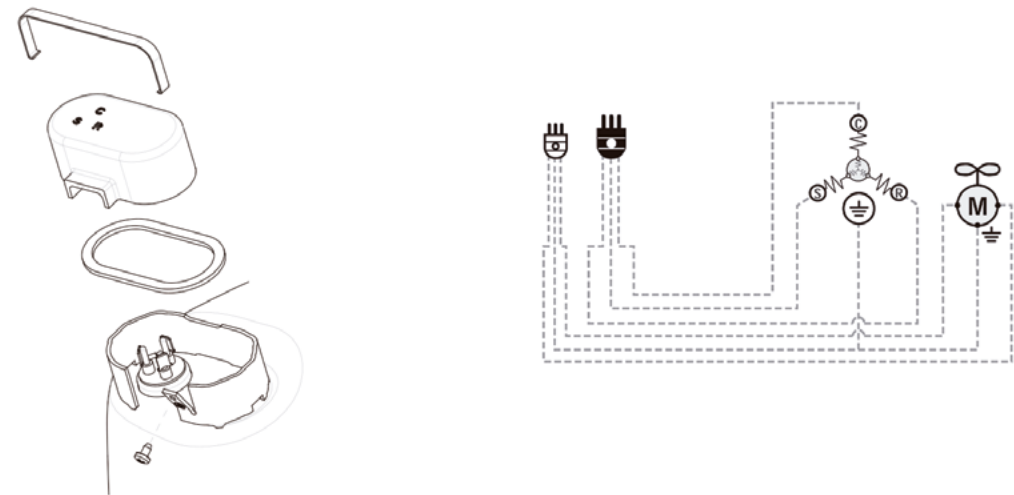
SM19 - NT SERIES CSIR Terminal Board
